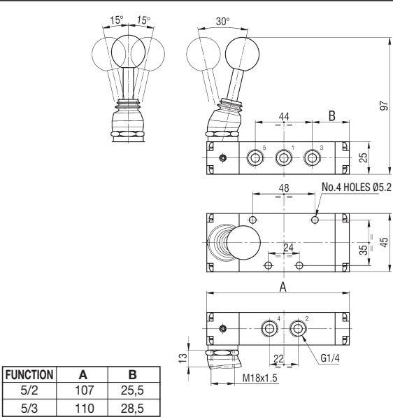
5/2 - 5/3 LATERAL KNOB
