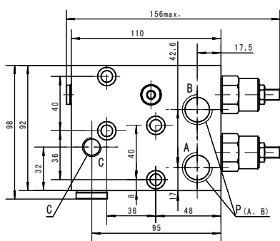
Overcenter valve FPRD
