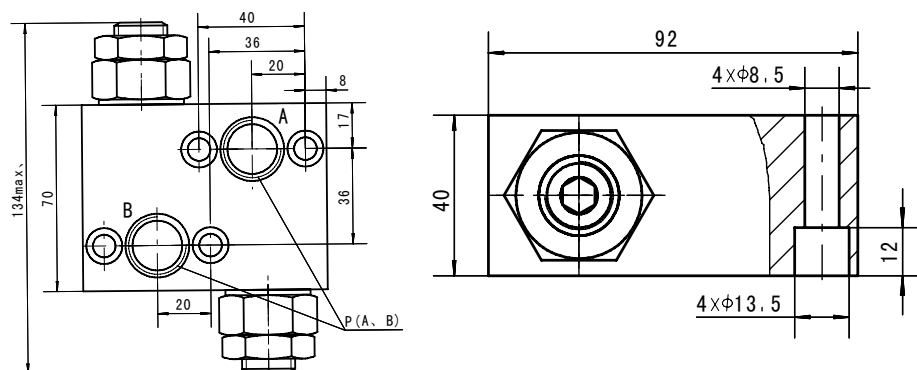
Dual grossover relief valve type FYRHD
