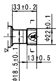
Shaft I: Splined 13-DP16/32
