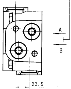
Porting ED 1-1/16-12UN O-ring 180° Apart ports
