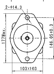
Flange WE
